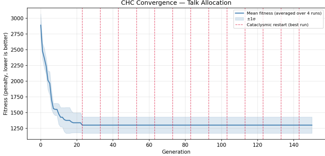
Figure 2: Average convergence over 4 runs on a synthetic instance ( T=18 , E=5 , R=30 , 150 generations, pop. 40). The shaded band shows \pm 1\sigma . Dashed vertical lines mark cataclysmic restarts of the best run.
